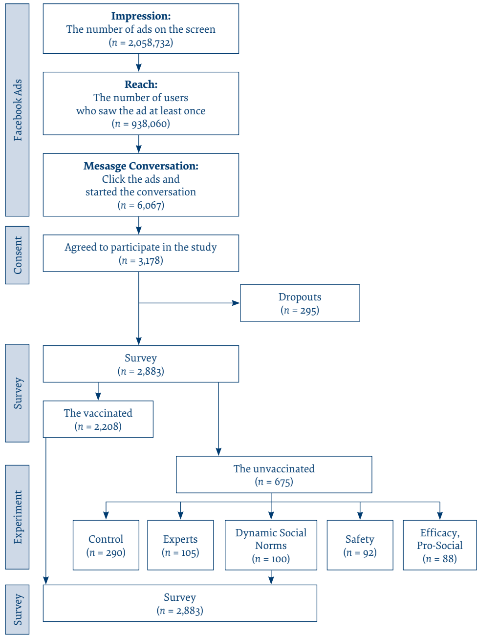
Figure 2. Study flowchart
